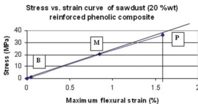
Figure 3 The stress vs. strain curve of sawdust (20% wt) reinforced phenolic composite. [Color figure can be viewed in the online issue, which is available at www.interscience.wiley.com .]
