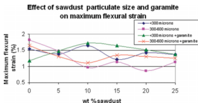
Figure 10 Maximum flexural strain of different percentages by weight and particle size of sawdust reinforced with phenolic resin with and without garamite. [Color figure can be viewed in the online issue, which is available at www.interscience.wiley.com .]
