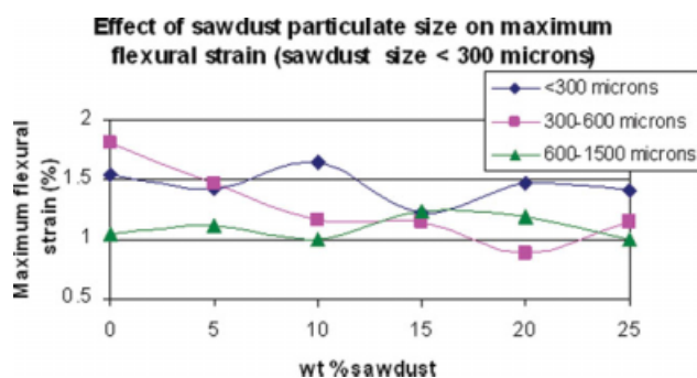
Figure 7 Strain of different percentages by weight of and particle size of sawdust reinforced with phenolic resin. [Color figure can be viewed in the online issue, which is available at www.interscience.wiley.com .]
