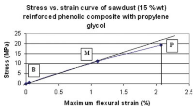
Figure 12 The stress vs. strain curve of sawdust (15% wt) reinforced phenolic composite with propylene glycol. [Color figure can be viewed in the online issue, which is available at www.interscience.wiley.com .]
