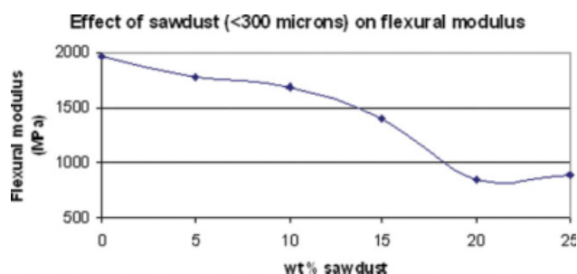
Figure 4 Flexural modulus of different percentage by weight of sawdust reinforced phenolic resin. [Color figure can be viewed in the online issue, which is available at www.interscience.wiley.com .]
