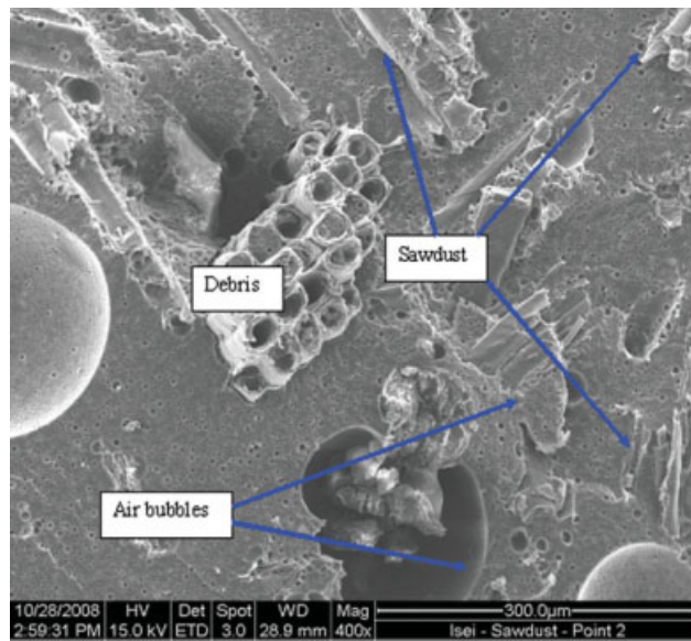
Figure 17 A closer look of the bottom left hand corner of Figure 16, 400 X. [Color figure can be viewed in the online issue, which is available at www.interscience.wiley.com .]
