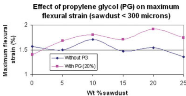
Figure 13 Maximum flexural strain of different percentages by weight of sawdust reinforced phenolic resin with and without propylene glycol (PG). [Color figure can be viewed in the online issue, which is available at www.interscience.wiley.com .]
