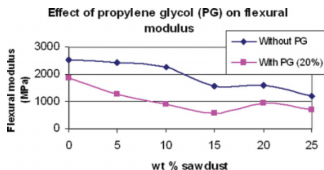
Figure 11 Flexural modulus of different percentages by weight of sawdust reinforced with phenolic resin with and without propylene glycol (PG). [Color figure can be viewed in the online issue, which is available at www.interscience.wiley.com .]
