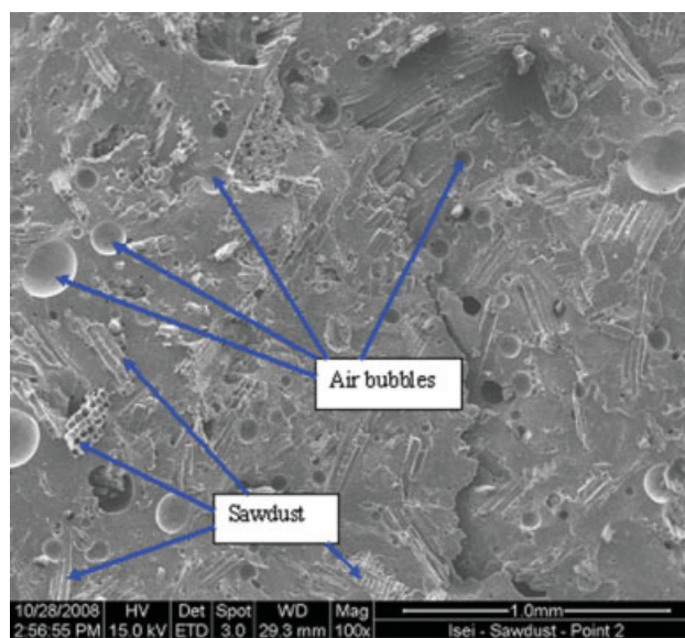
Figure 16 Fractured surface of 15% by weight of sawdust (<300 μm) reinforced phenolic composite, 100 X. [Color figure can be viewed in the online issue, which is available at www.interscience.wiley.com .]
