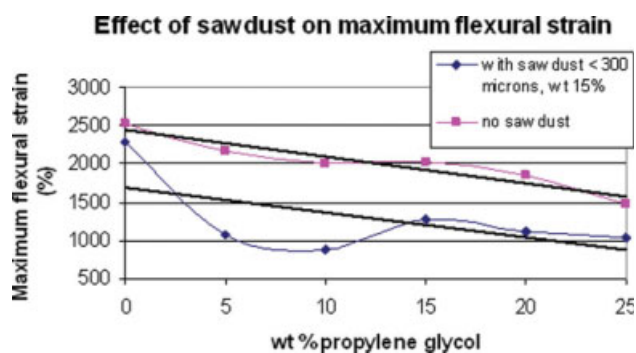
Figure 14 Maximum flexural strain of different percentages by weight of propylene glycol plus 1% garamite reinforced phenolic resin with and without sawdust. [Color figure can be viewed in the online issue, which is available at www.interscience.wiley.com .]
