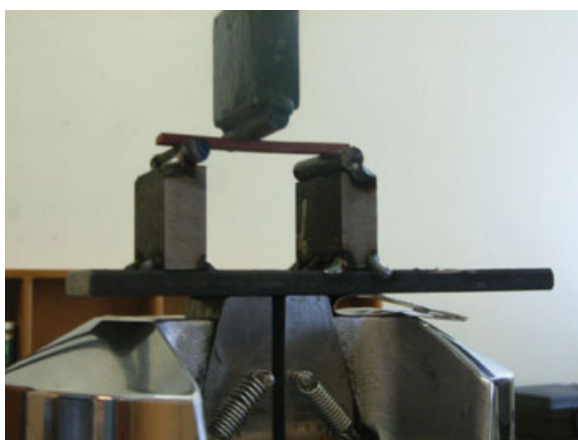
Figure 2 Three-point bending test on flexural specimen. [Color figure can be viewed in the online issue, which is available at www.interscience.wiley.com .]
