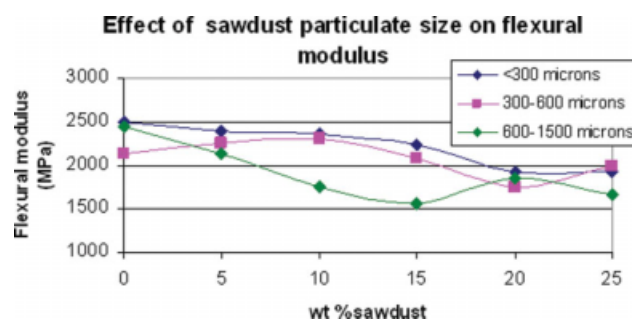
Figure 5 Flexural modulus of different percentages by weight and particulate sizes of sawdust reinforced phenolic resin. [Color figure can be viewed in the online issue, which is available at www.interscience.wiley.com .]
