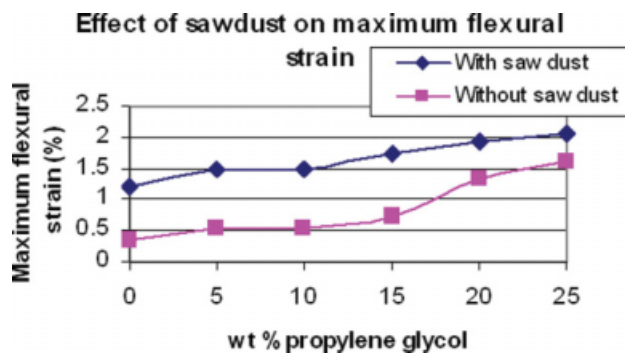
Figure 15 Maximum flexural strain of different percentages by weight of propylene glycol plus 1% garamite reinforced phenolic resin with and without sawdust. [Color figure can be viewed in the online issue, which is available at www.interscience.wiley.com .]
