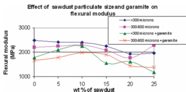
Figure 9 Flexural modulus of different percentages by weight and particle sizes of sawdust reinforced with phenolic resin with and without garamite. [Color figure can be viewed in the online issue, which is available at www.interscience.wiley.com .]
